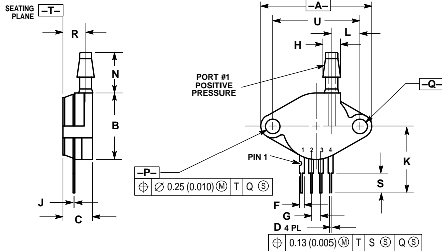
Figure 3. Case Outline Drawings Top: Case 371D-02, Issue B Bottom: Case 350-03, Issue H
