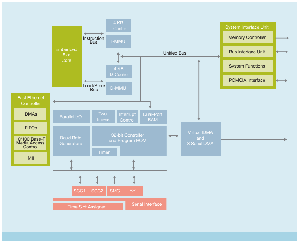
MPC853T Block Diagram
